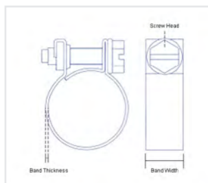
W1 - Zinc Plated Mild Steel Band, Screw & Nut W4 - Stainless Steel Band, Screw & Nut
